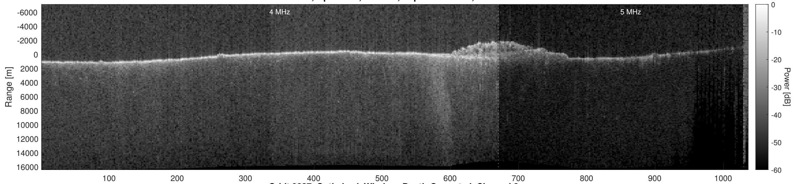
Orbit 9837, Optimized, Window, Depth-Corrected, Channel 2
