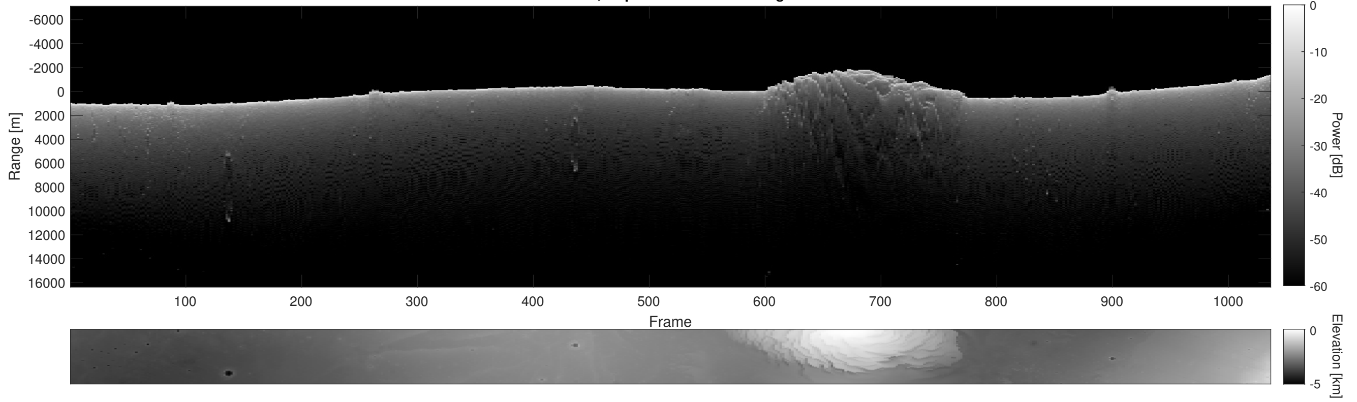
Orbit 9837, Depth-Corrected Cluttergram
