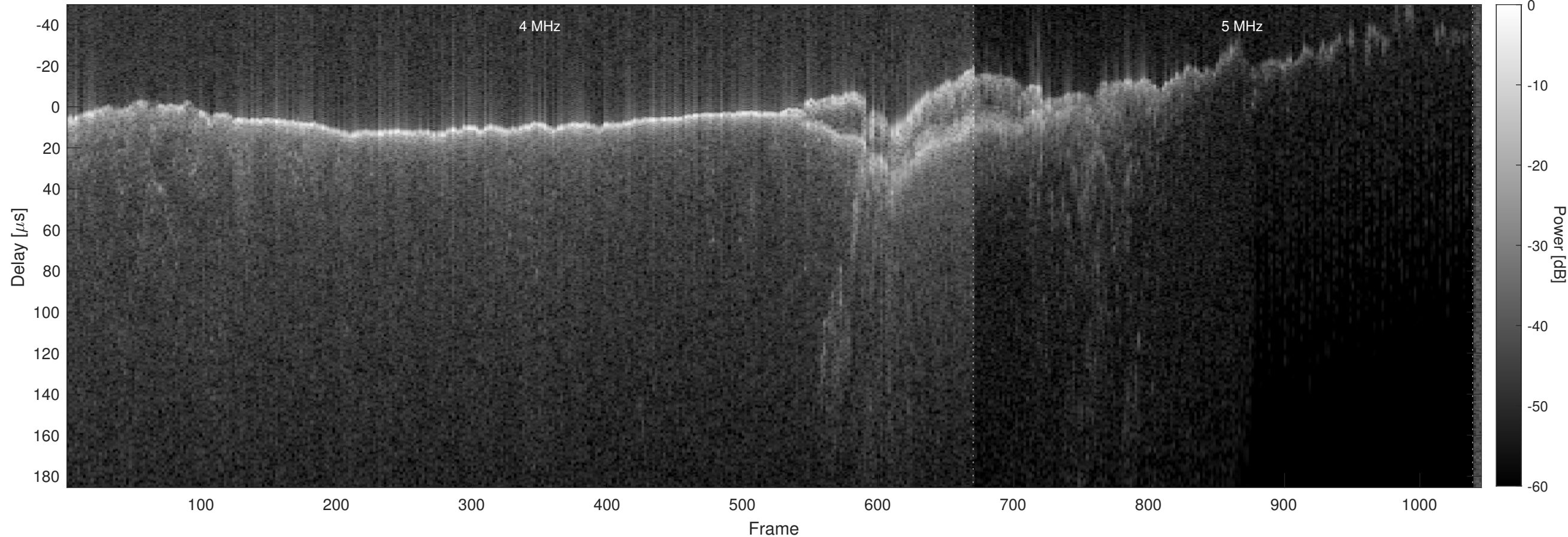
Orbit 9838, Chapman, No Window, Channel 2
