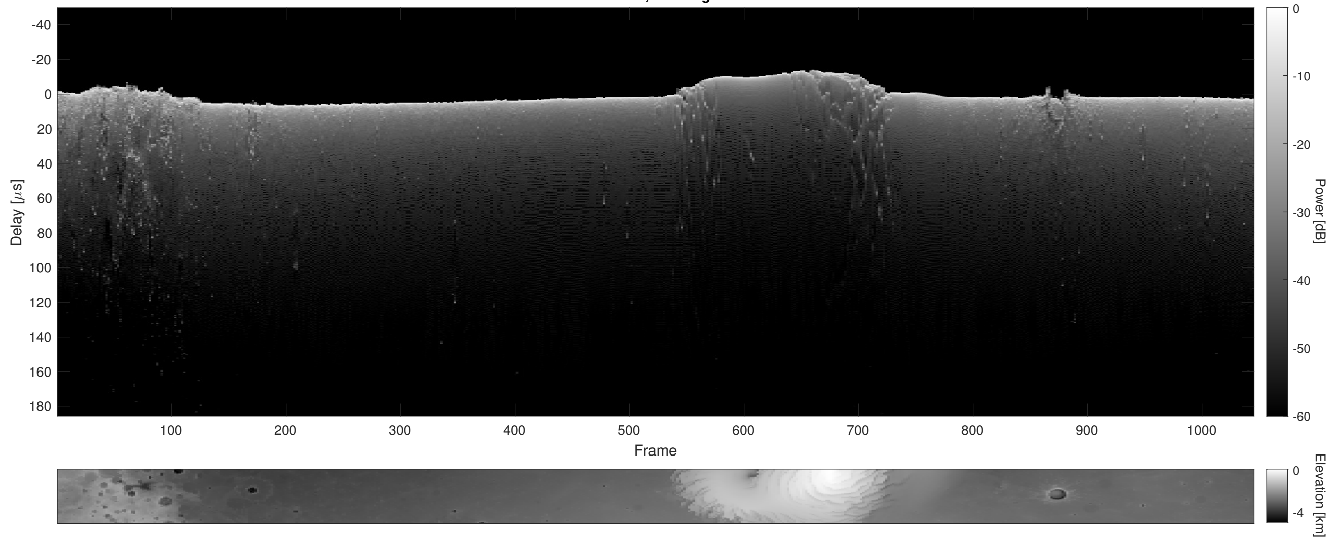
Orbit 9838, Cluttergram
