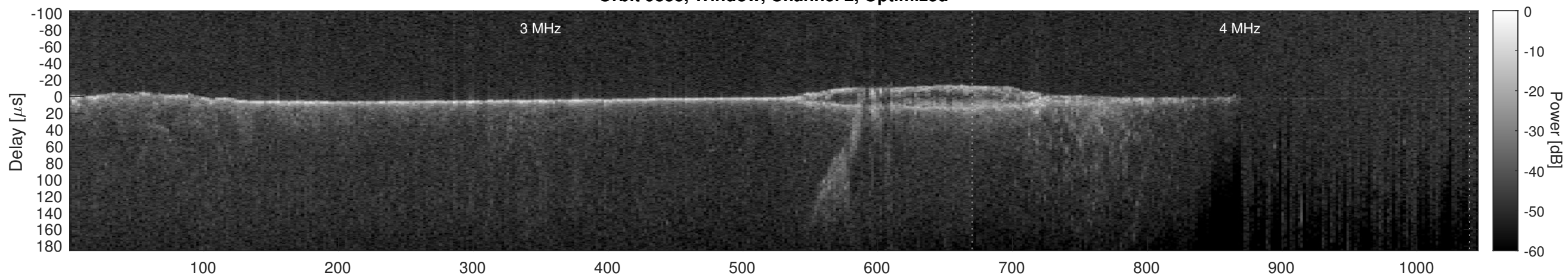
Orbit 9838, Cluttergram
