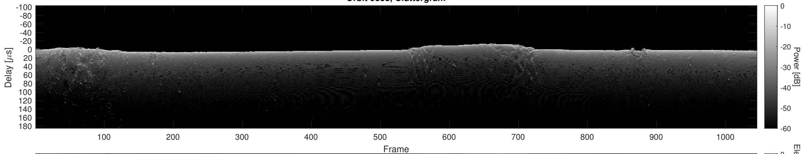
Orbit 9838, Cluttergram
