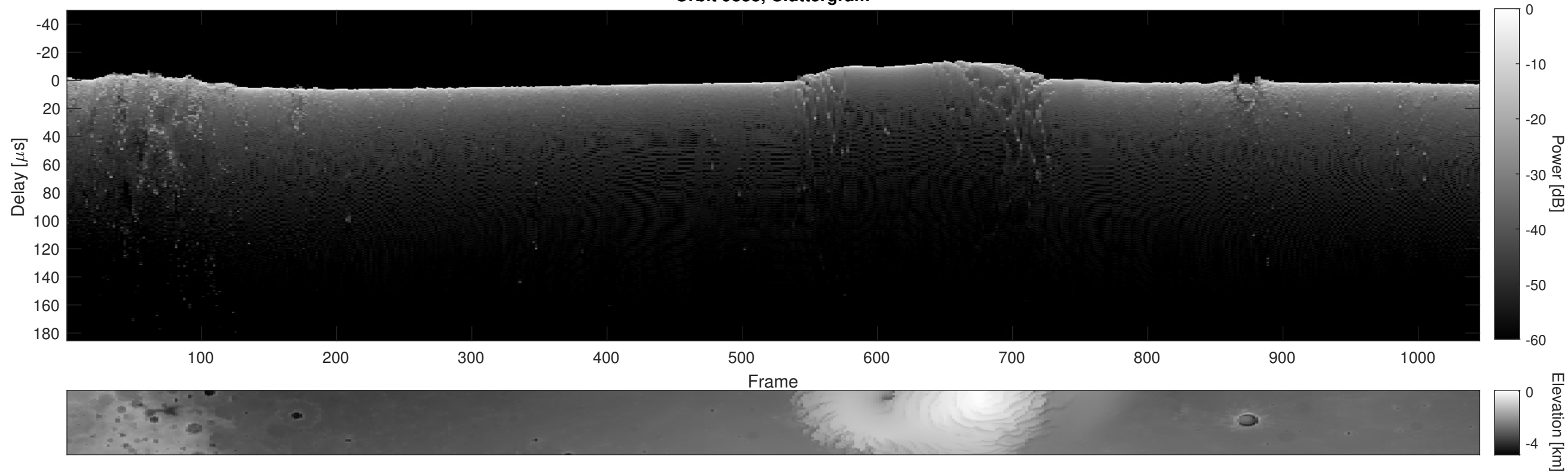
Orbit 9838, Cluttergram
