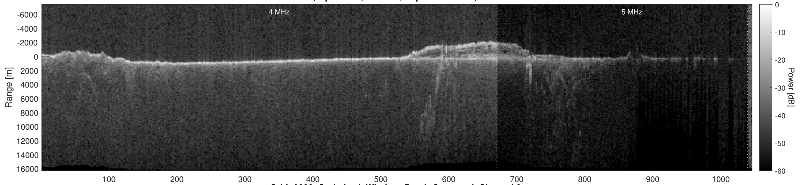
Orbit 9838, Optimized, Window, Depth-Corrected, Channel 2
