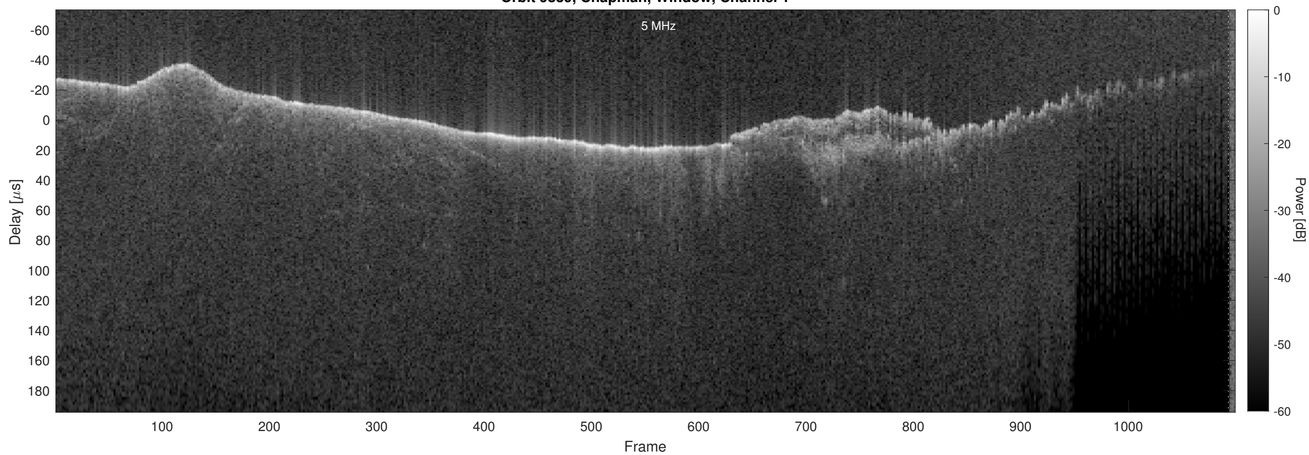
Orbit 9839, Chapman, Window, Channel 2
