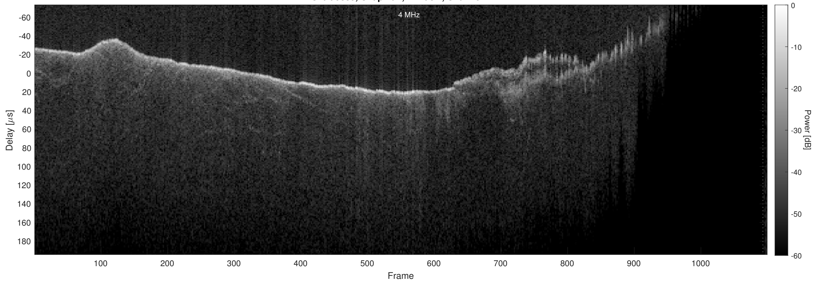
Orbit 9839, Chapman, Window, Channel 2
