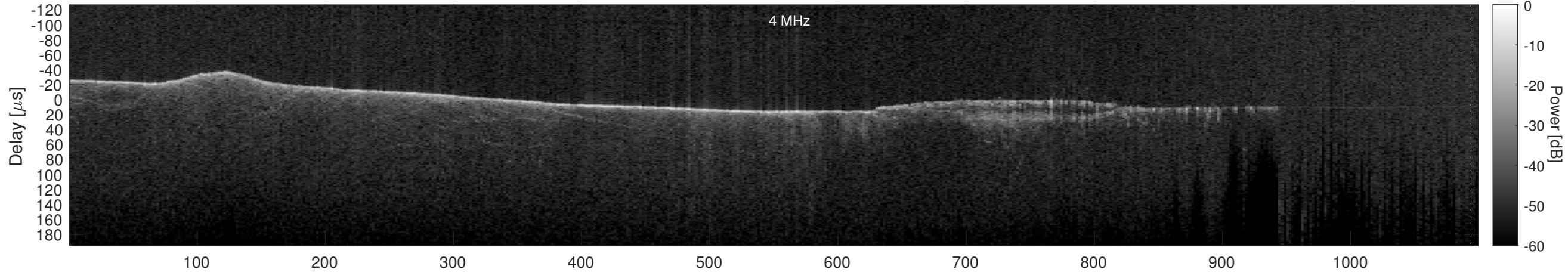
Orbit 9839, Cluttergram
