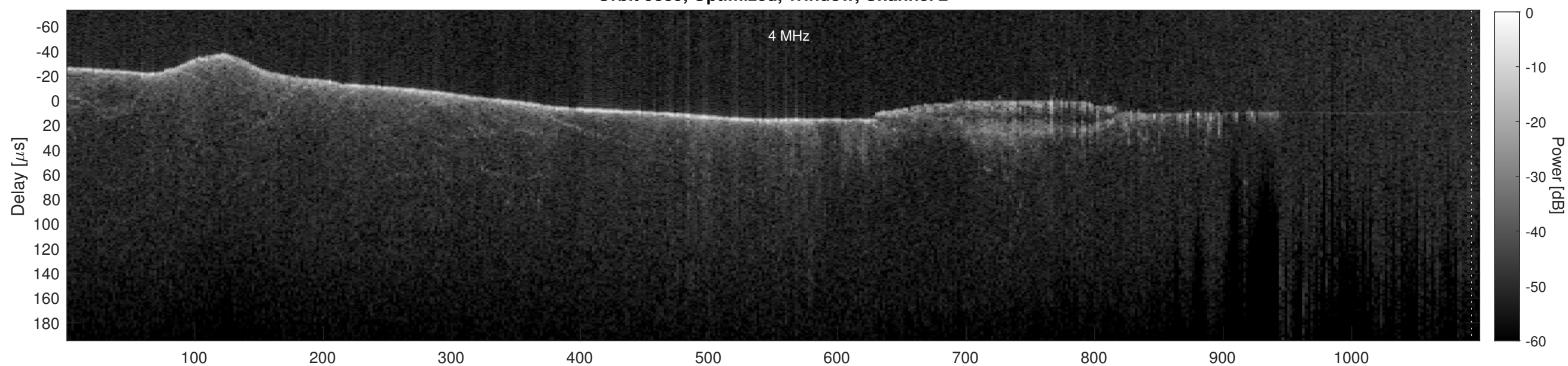
Orbit 9839, Cluttergram
