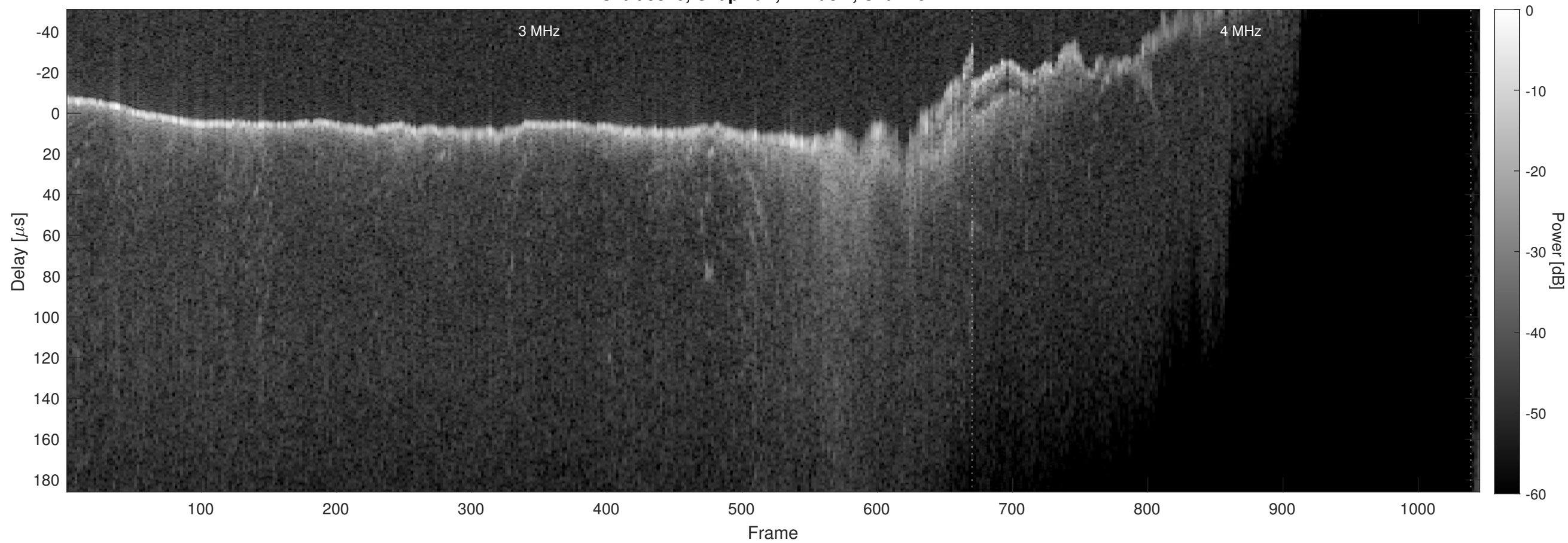
Orbit 9840, Chapman, Window, Channel 2
