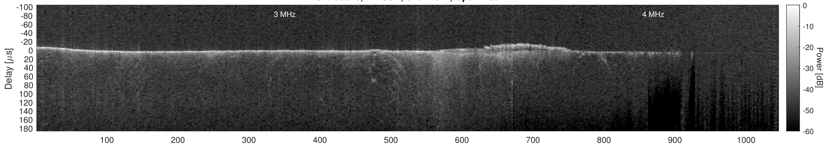
Orbit 9840, Cluttergram
