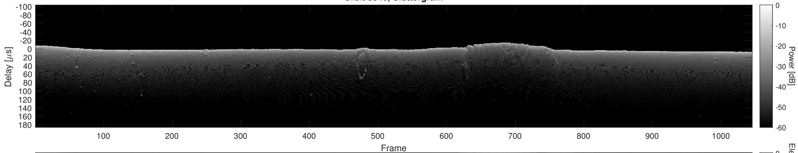
Orbit 9840, Cluttergram
