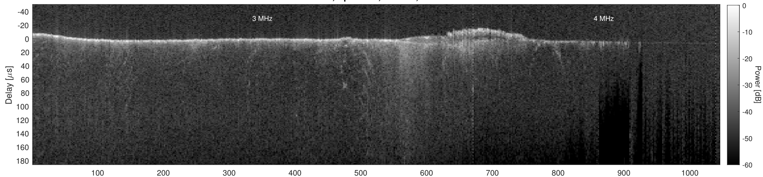
Orbit 9840, Cluttergram
