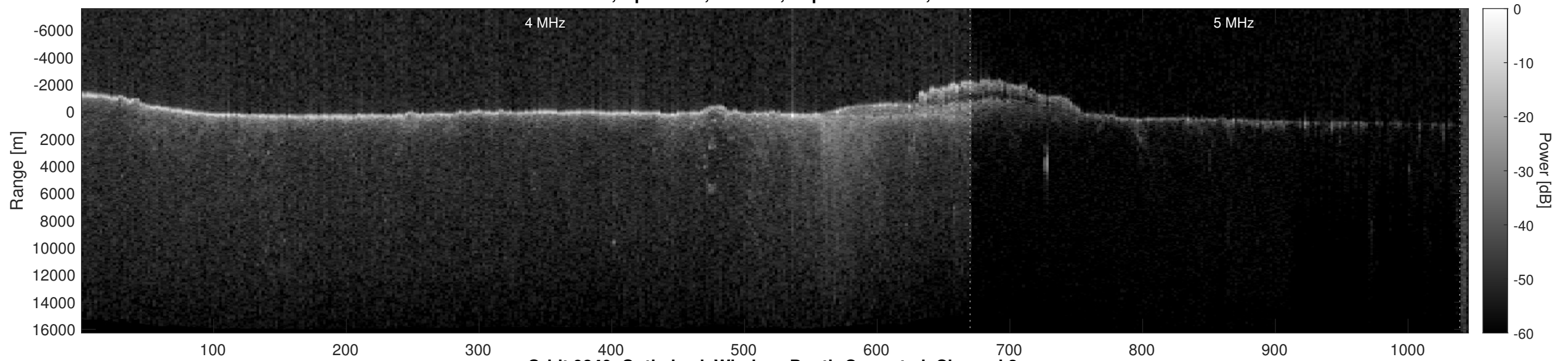
Orbit 9840, Optimized, Window, Depth-Corrected, Channel 2
