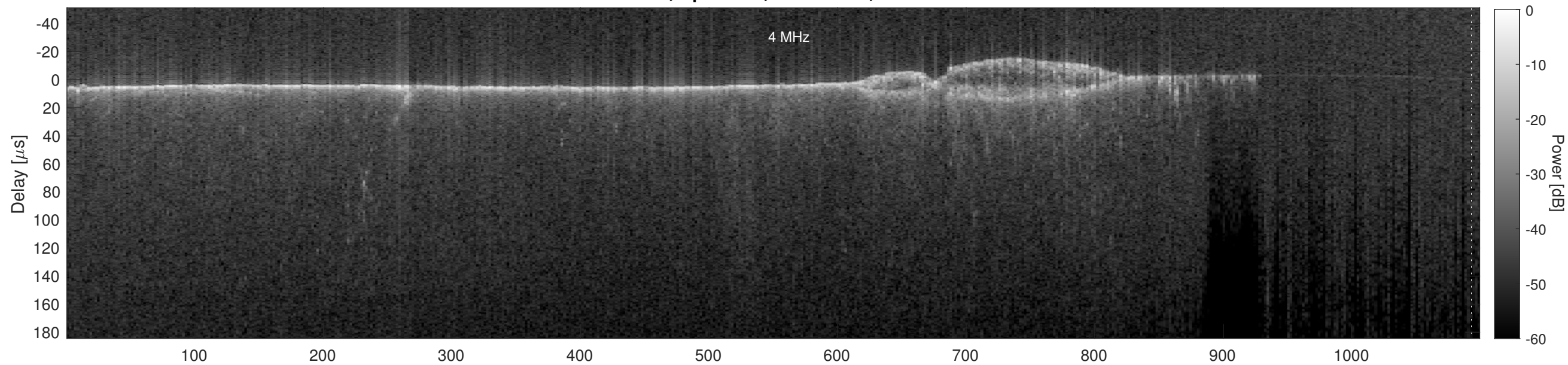
Orbit 9842, Cluttergram
