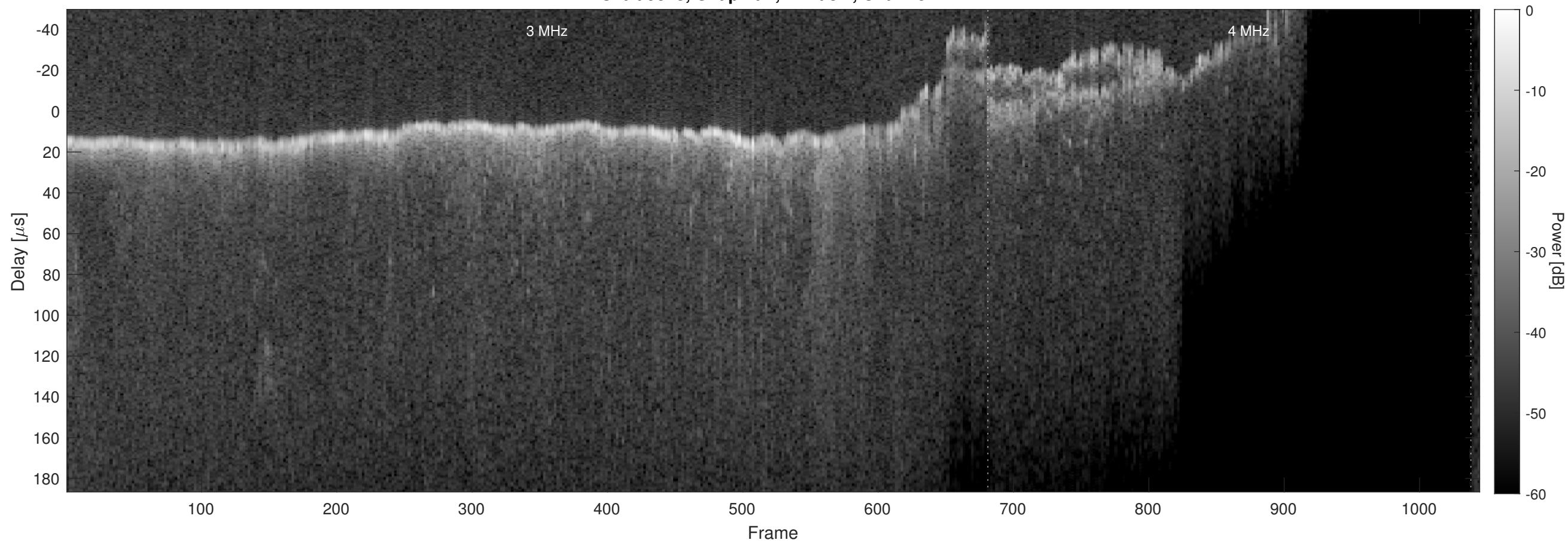
Orbit 9843, Chapman, Window, Channel 2
