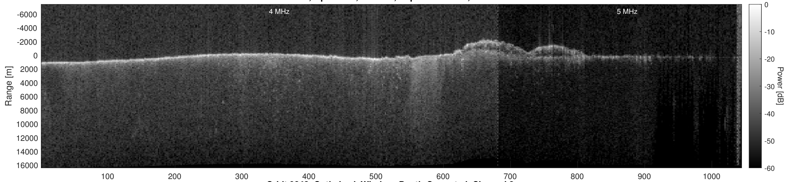
Orbit 9843, Optimized, Window, Depth-Corrected, Channel 2
