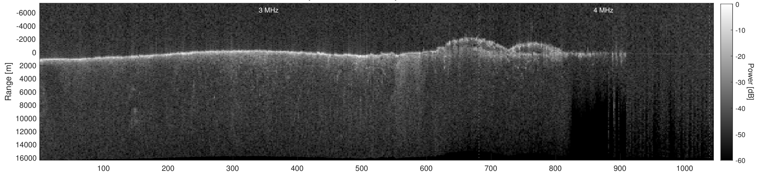
Orbit 9843, Depth-Corrected Cluttergram
