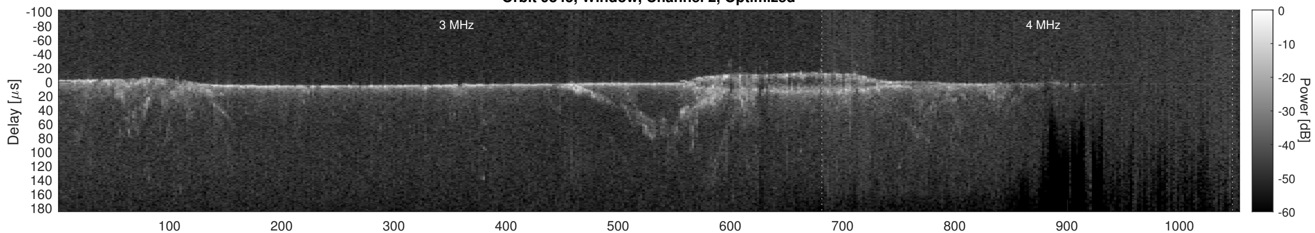
Orbit 9845, Cluttergram
