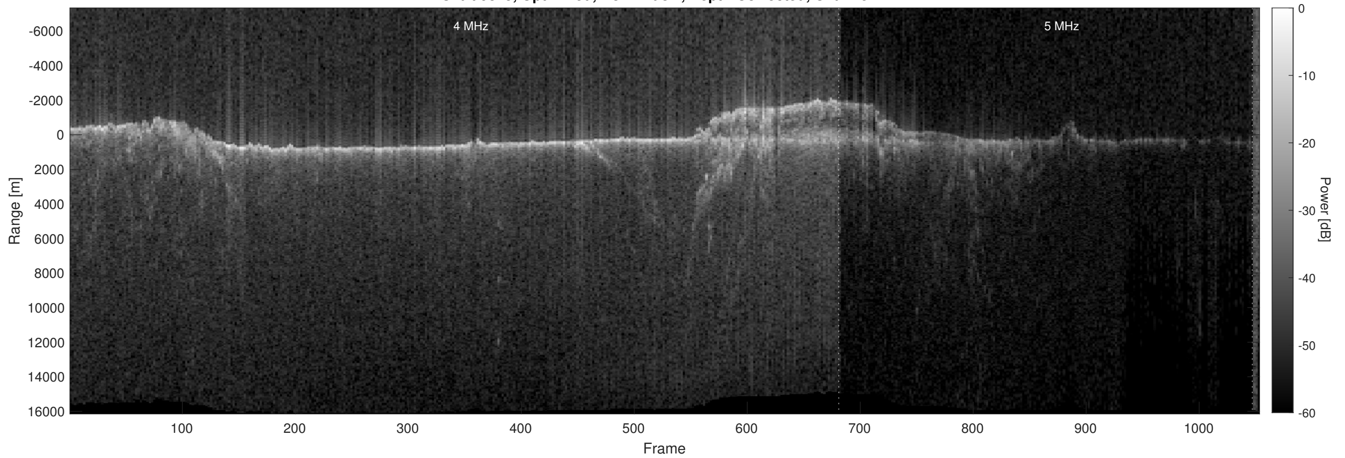
Orbit 9845, Optimized, No Window, Depth-Corrected, Channel 2
