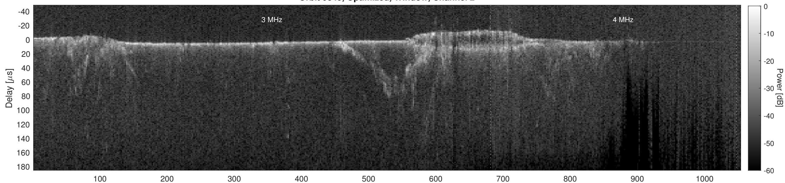
Orbit 9845, Cluttergram
