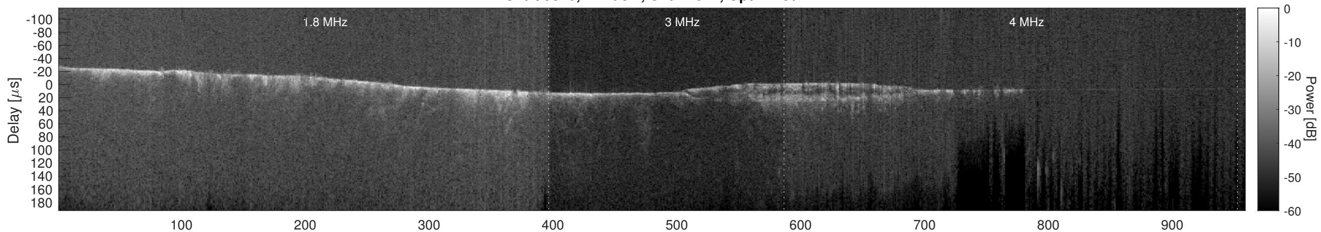
Orbit 9846, Cluttergram
