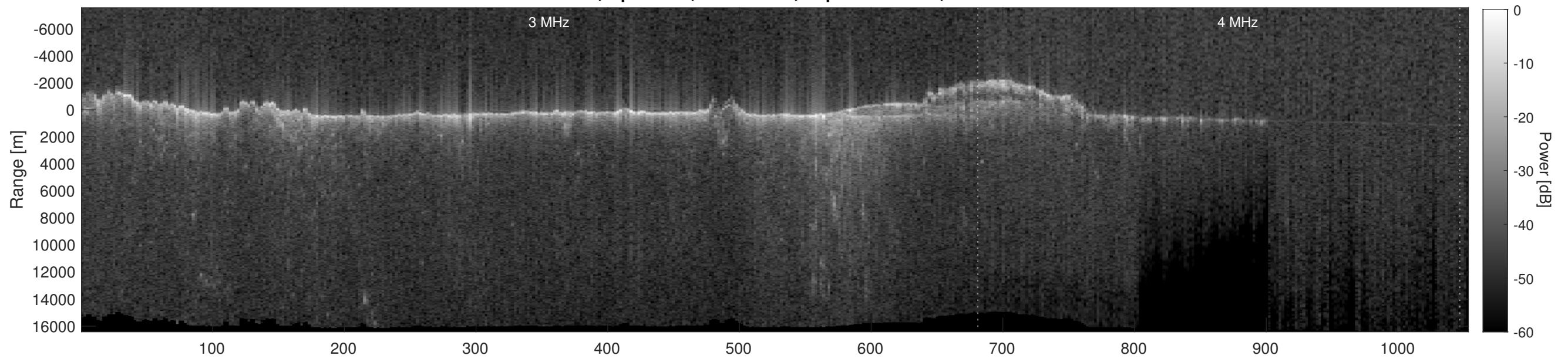
Orbit 9847, Depth-Corrected Cluttergram
