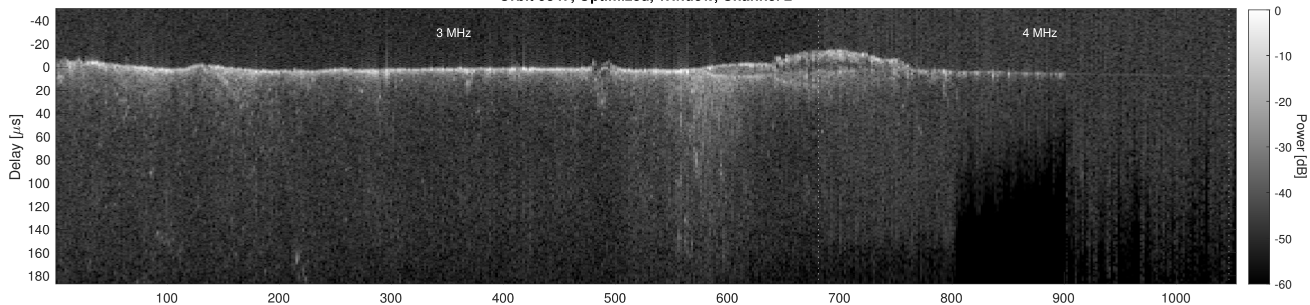
Orbit 9847, Cluttergram
