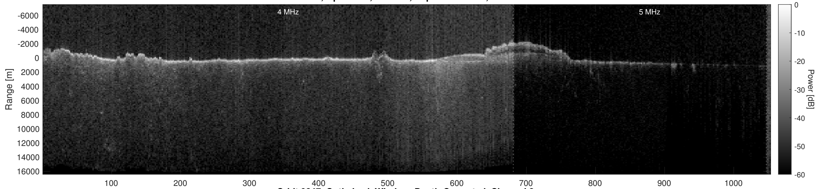
Orbit 9847, Optimized, Window, Depth-Corrected, Channel 2
