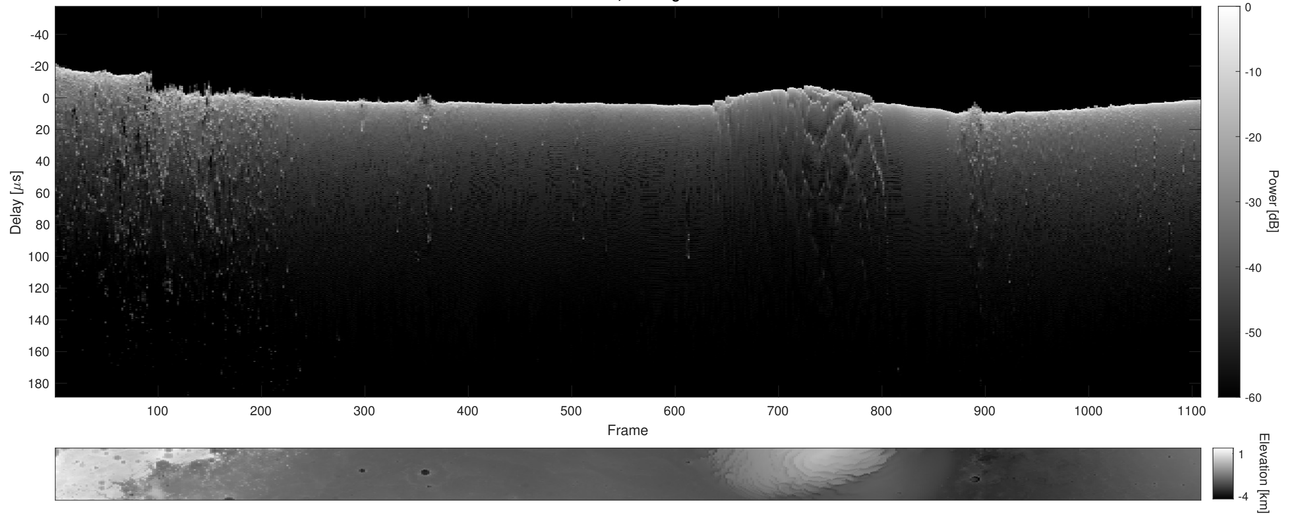
Orbit 9848, Cluttergram
