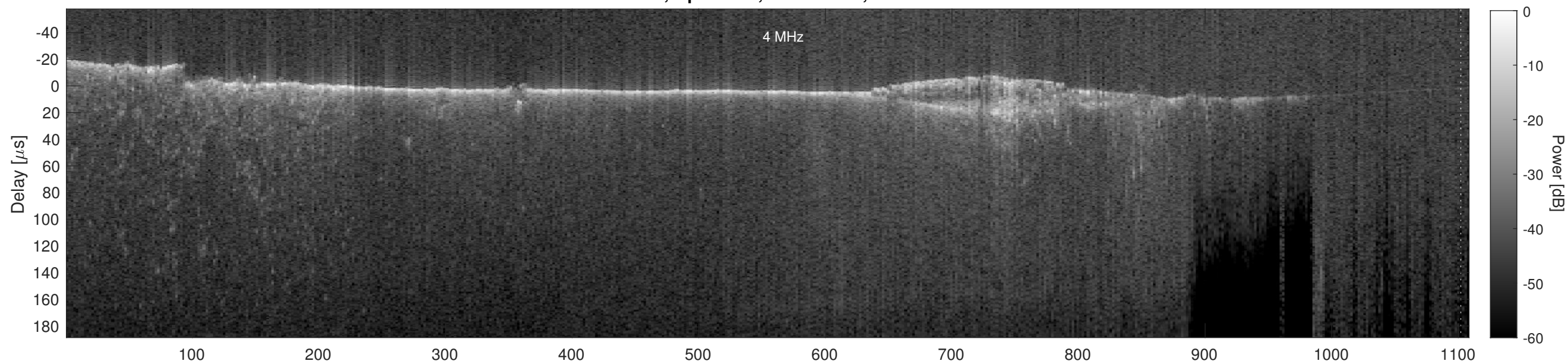
Orbit 9848, Cluttergram
