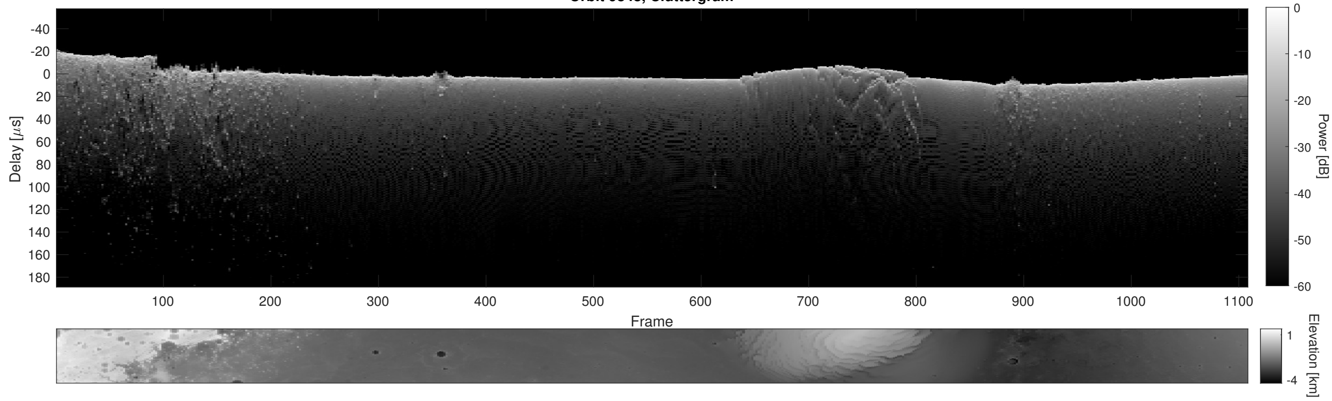
Orbit 9848, Cluttergram
