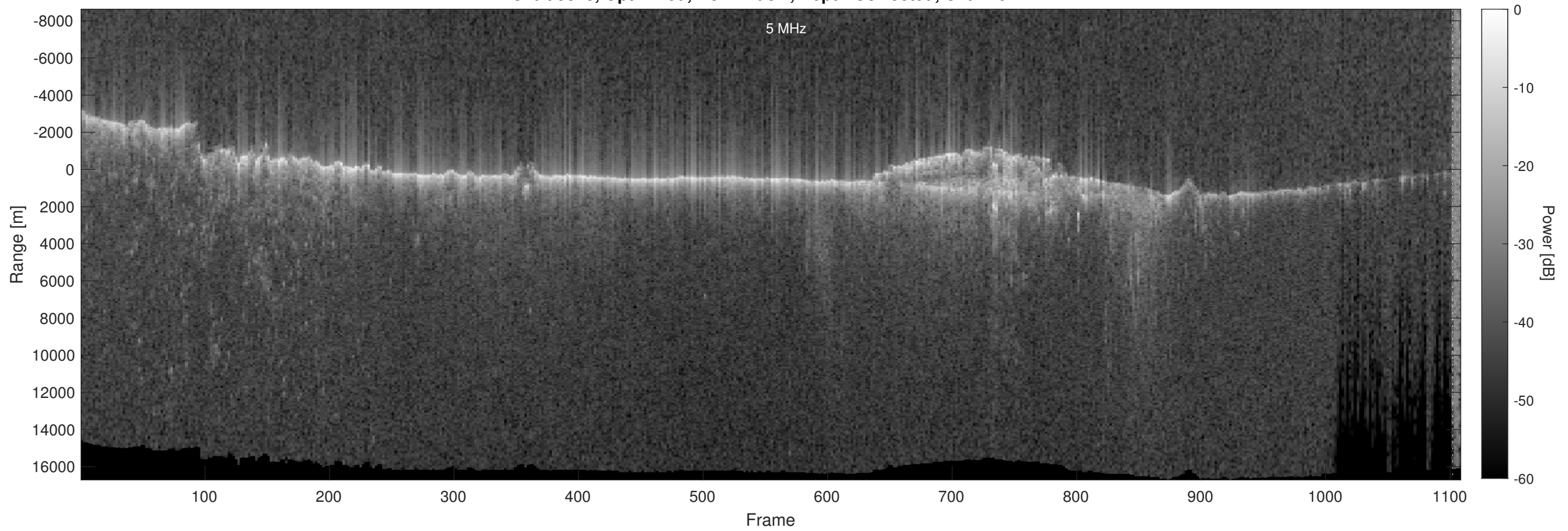
Orbit 9848, Optimized, No Window, Depth-Corrected, Channel 2
