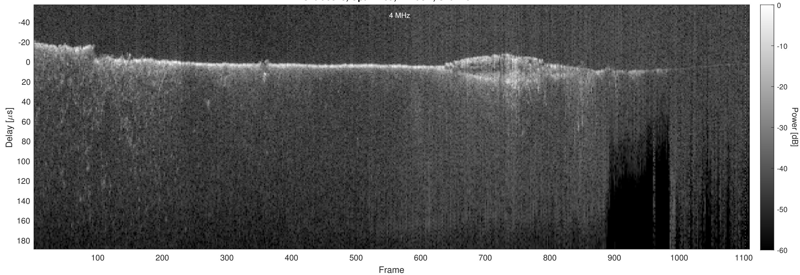
Orbit 9848, Optimized, Window, Channel 2
