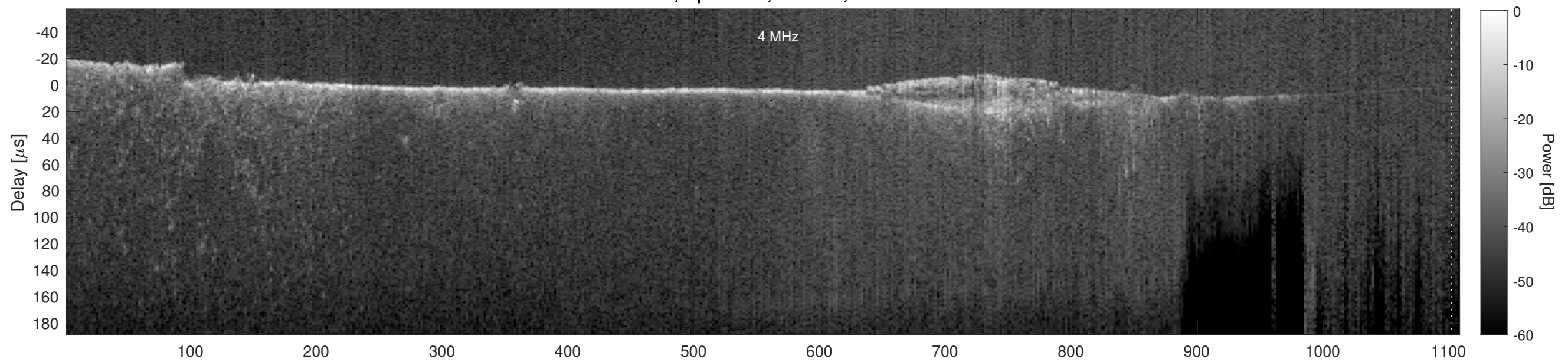
Orbit 9848, Cluttergram
