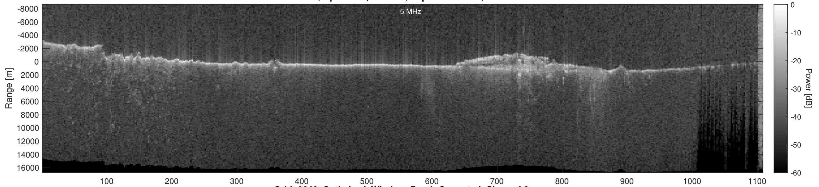
Orbit 9848, Optimized, Window, Depth-Corrected, Channel 2
