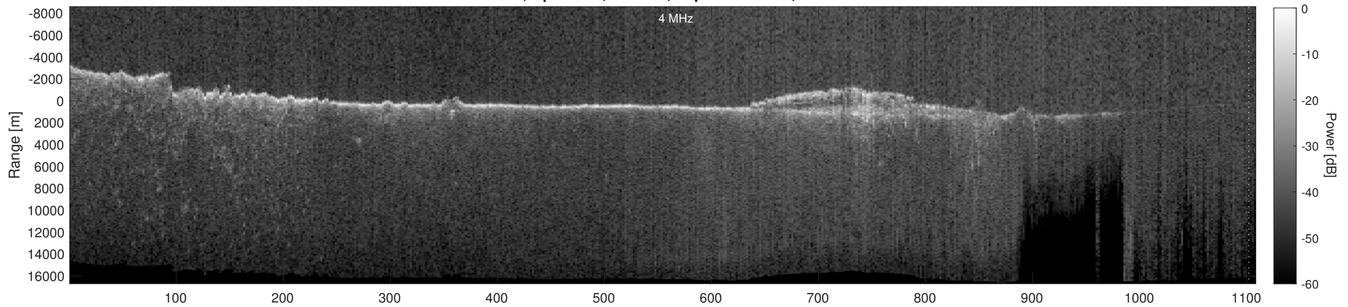
Orbit 9848, Depth-Corrected Cluttergram
