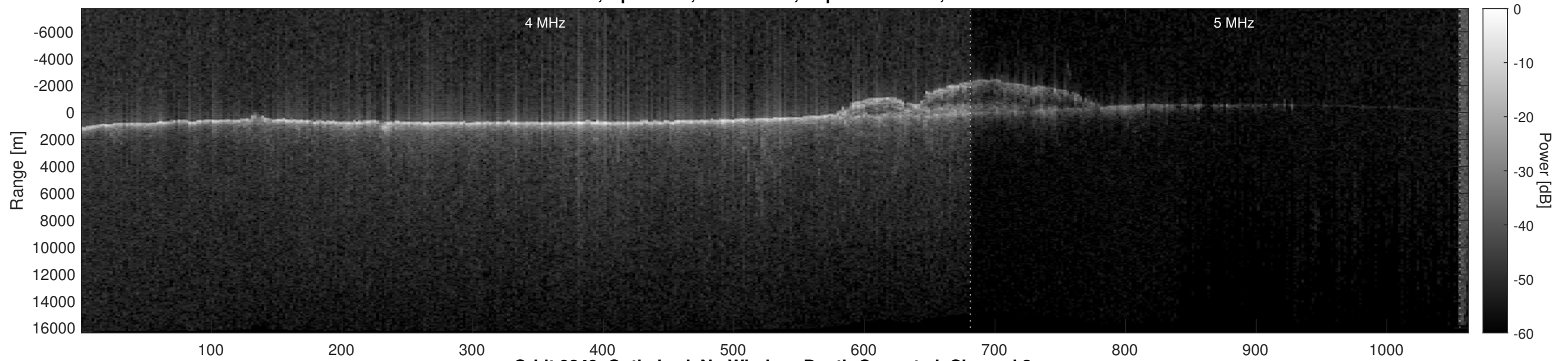
Orbit 9849, Optimized, No Window, Depth-Corrected, Channel 2
