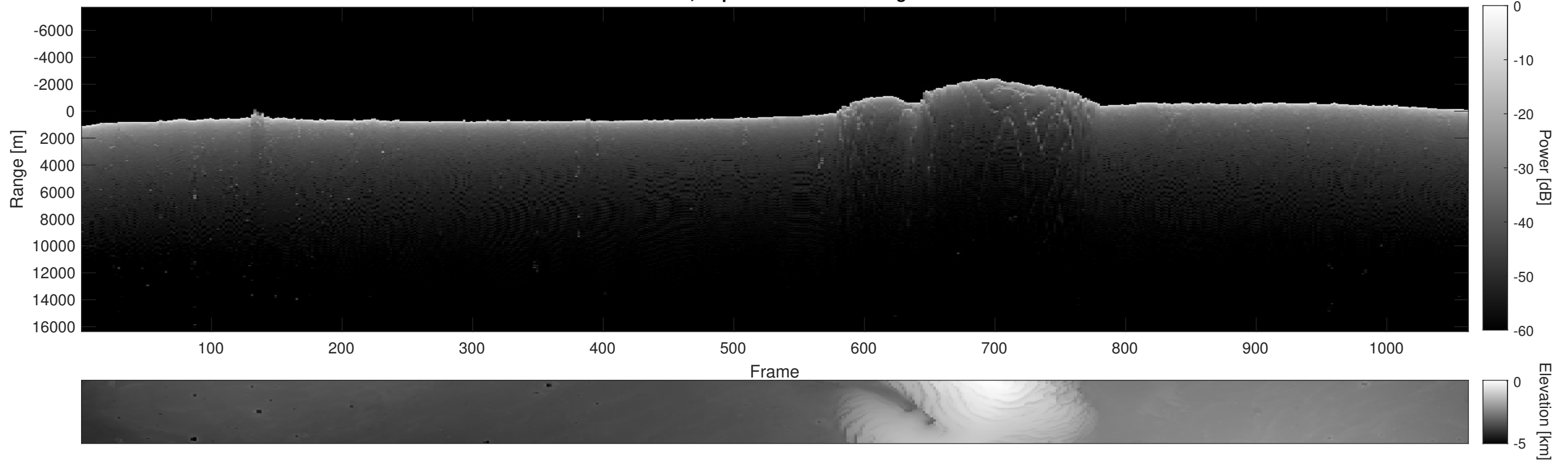
Orbit 9849, Depth-Corrected Cluttergram
