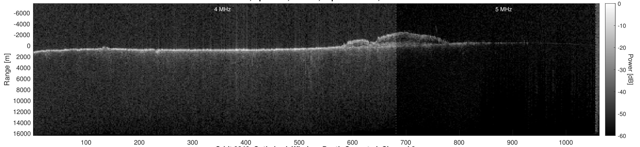
Orbit 9849, Optimized, Window, Depth-Corrected, Channel 2
