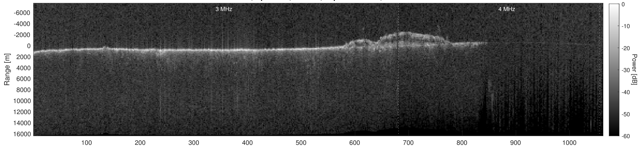
Orbit 9849, Depth-Corrected Cluttergram
