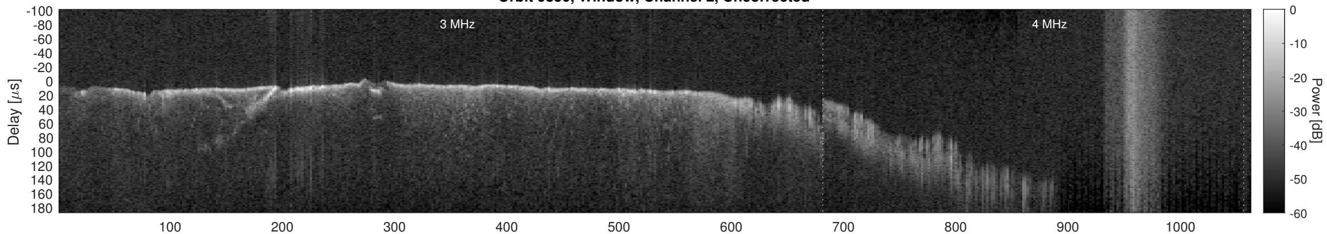
Orbit 9850, Window, Channel 2, Chapman
