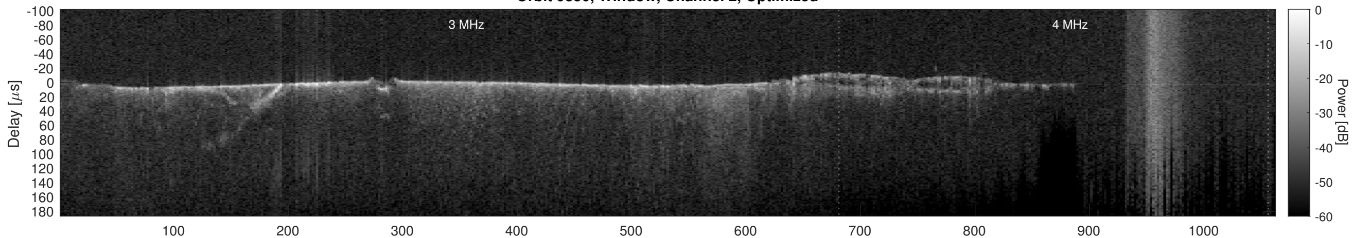
Orbit 9850, Cluttergram
