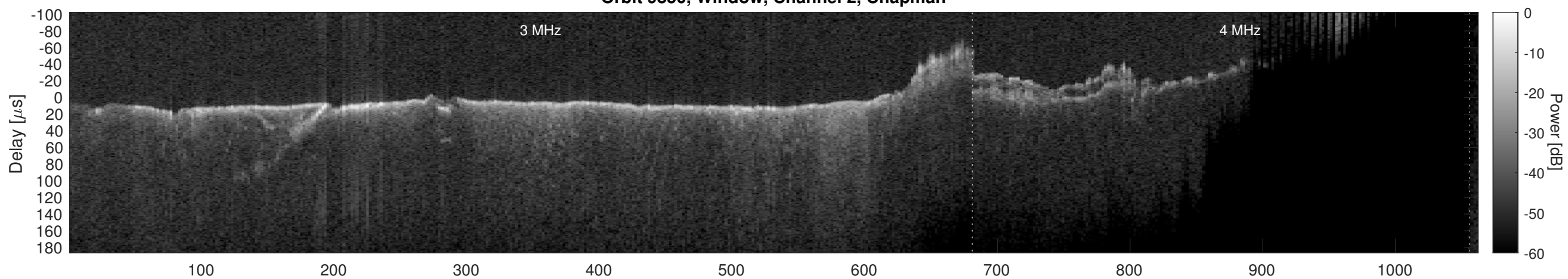
Orbit 9850, Window, Channel 2, Optimized
