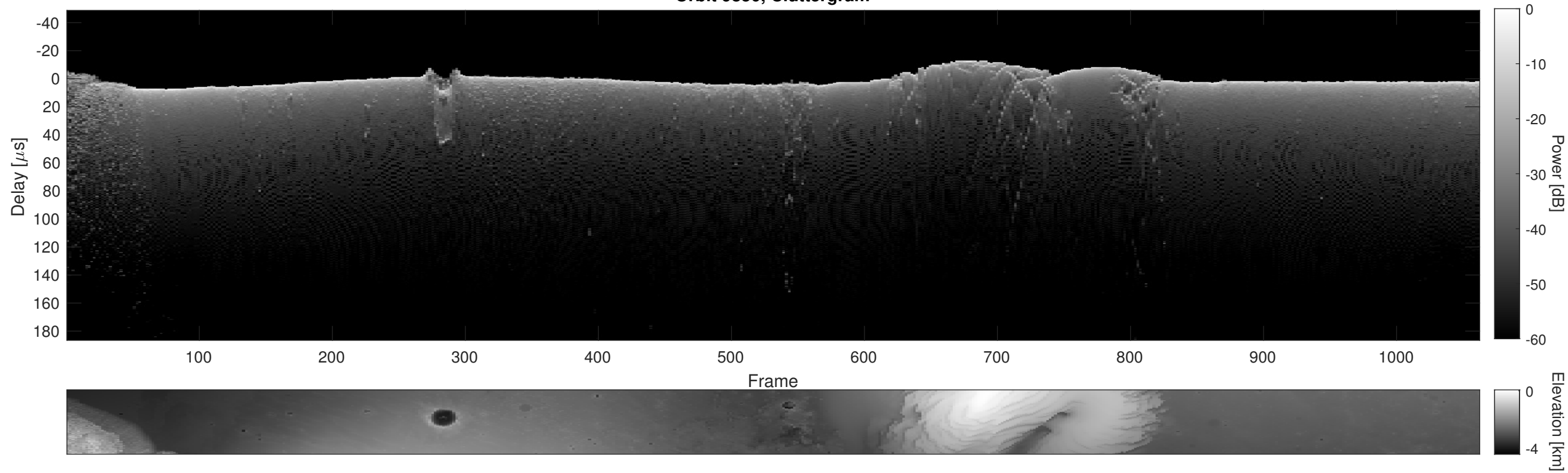
Orbit 9850, Cluttergram
