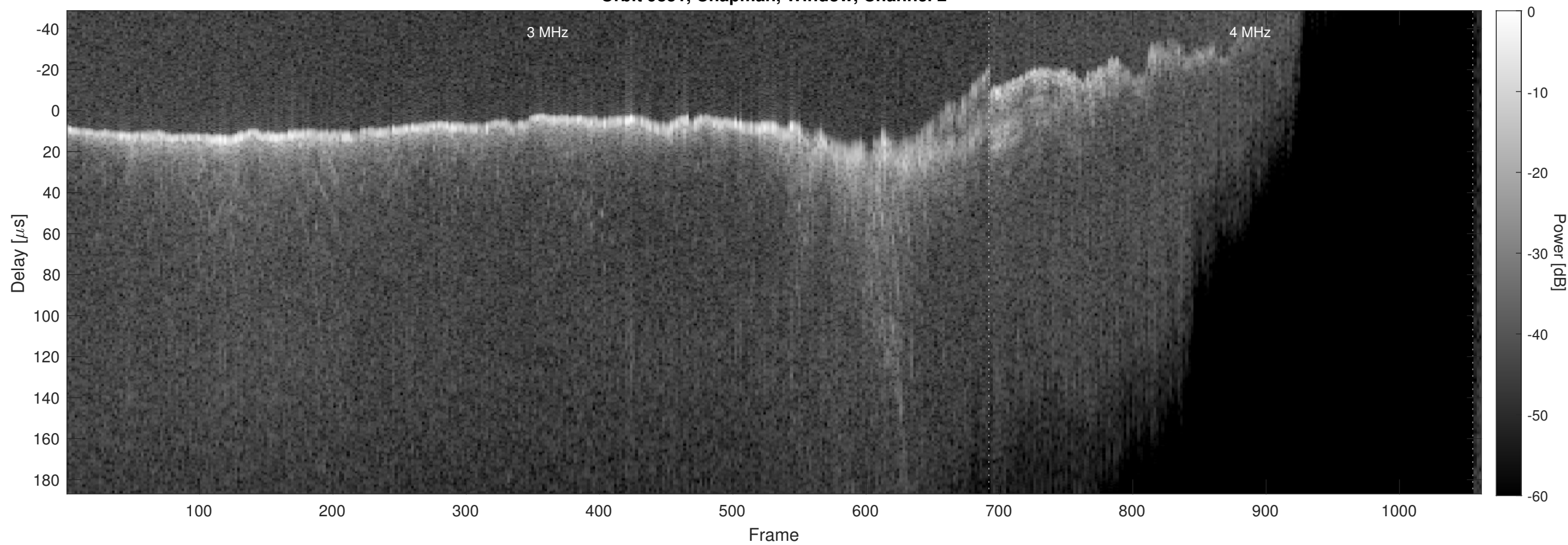
Orbit 9851, Chapman, Window, Channel 2
