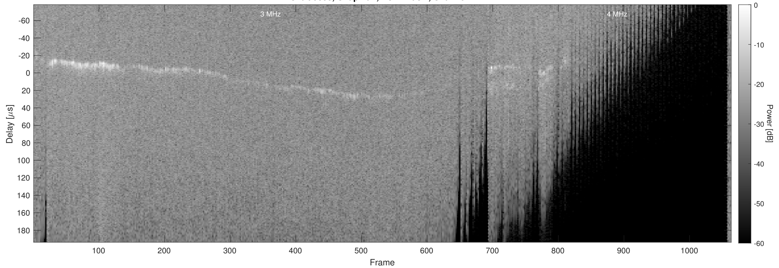
Orbit 9853, Chapman, No Window, Channel 2
