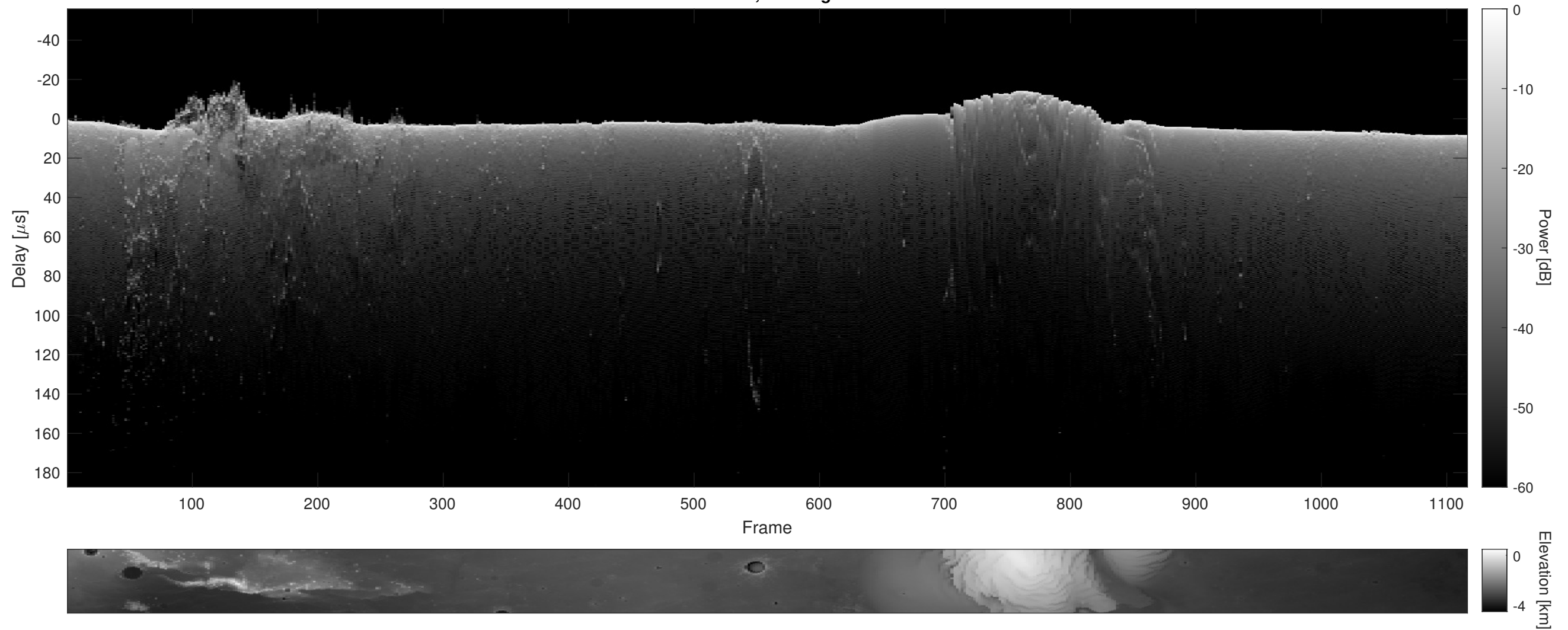
Orbit 9854, Cluttergram
