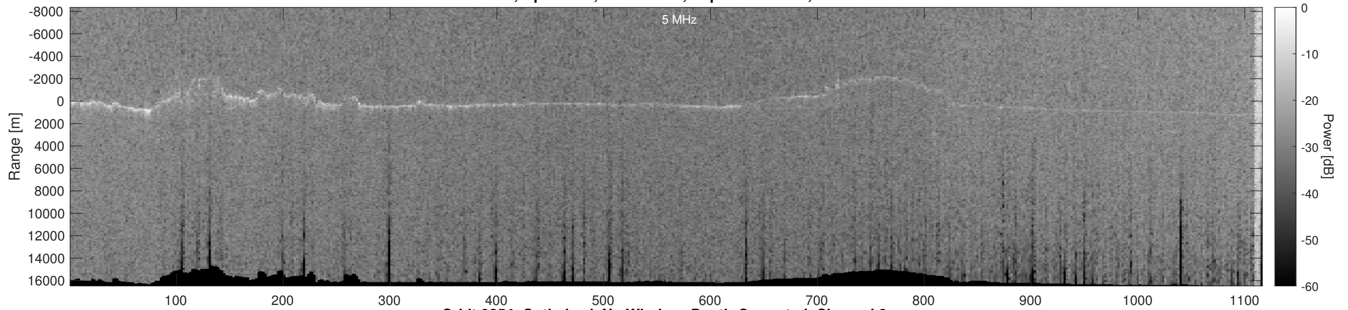
Orbit 9854, Optimized, No Window, Depth-Corrected, Channel 2
