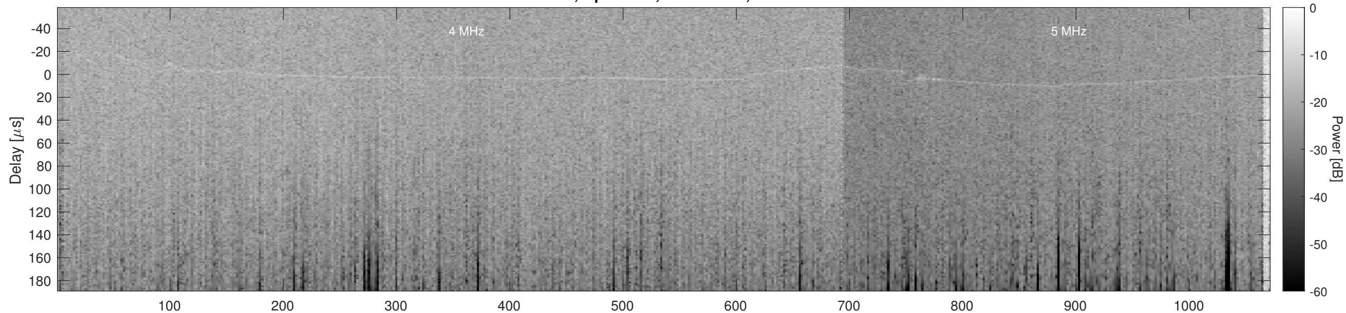
Orbit 9855, Optimized, No Window, Channel 2
