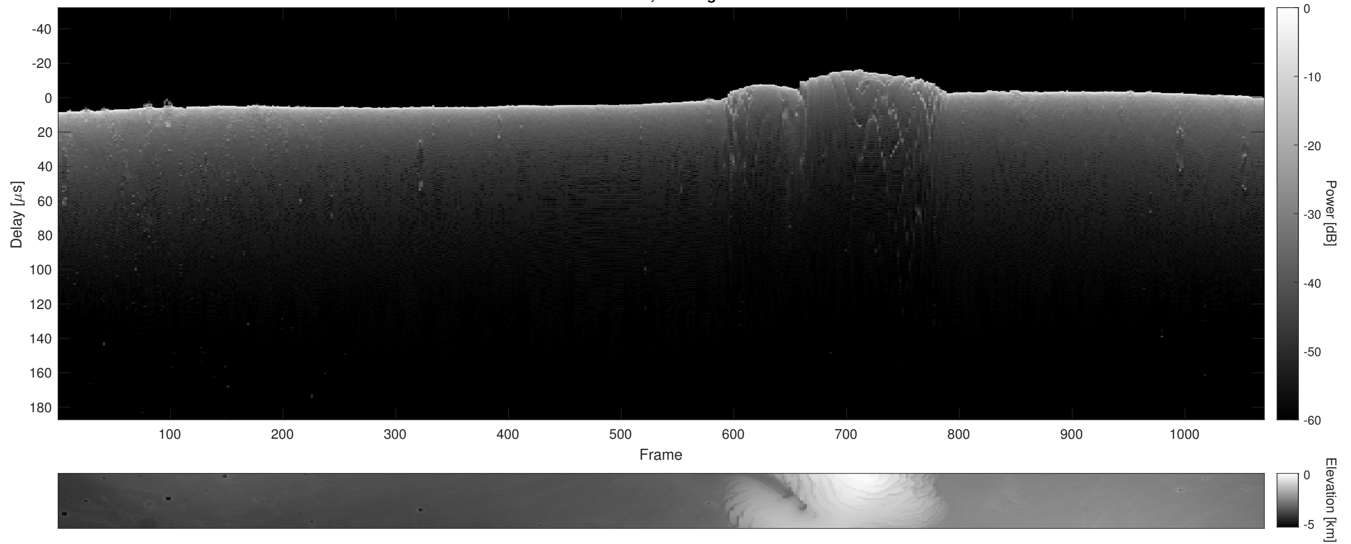
Orbit 9856, Cluttergram
