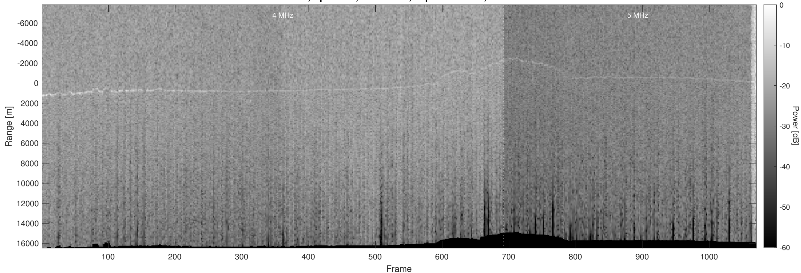
Orbit 9856, Optimized, No Window, Depth-Corrected, Channel 2
