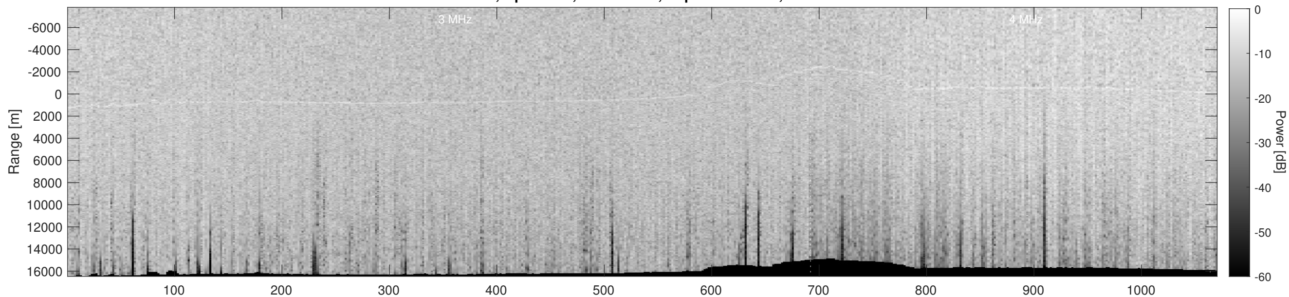
Orbit 9856, Depth-Corrected Cluttergram
