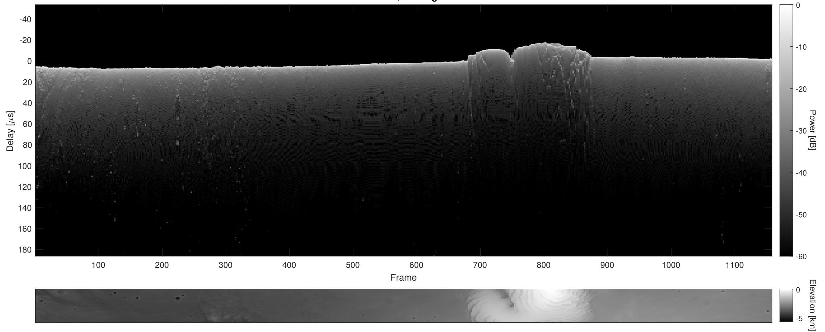
Orbit 9877, Cluttergram
