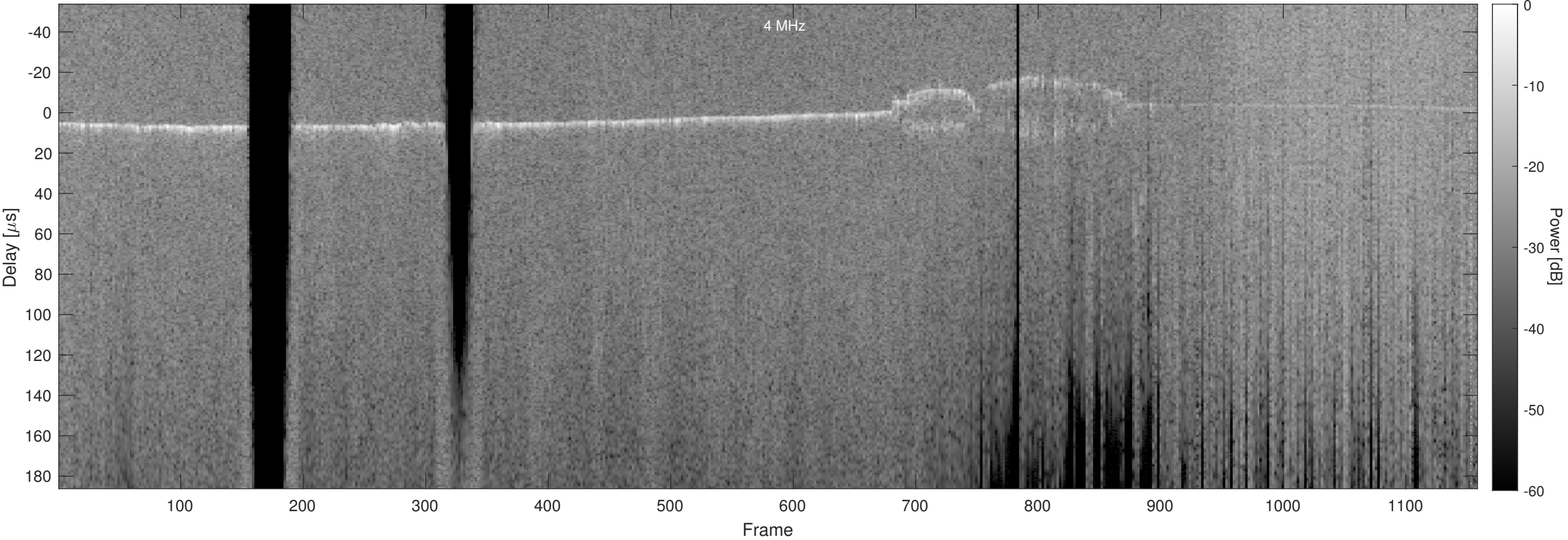
Orbit 9877, Optimized, No Window, Channel 2
