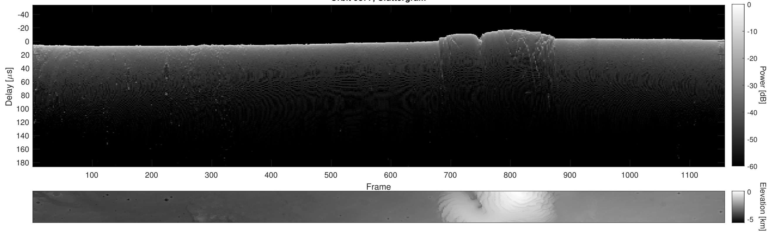
Orbit 9877, Cluttergram
