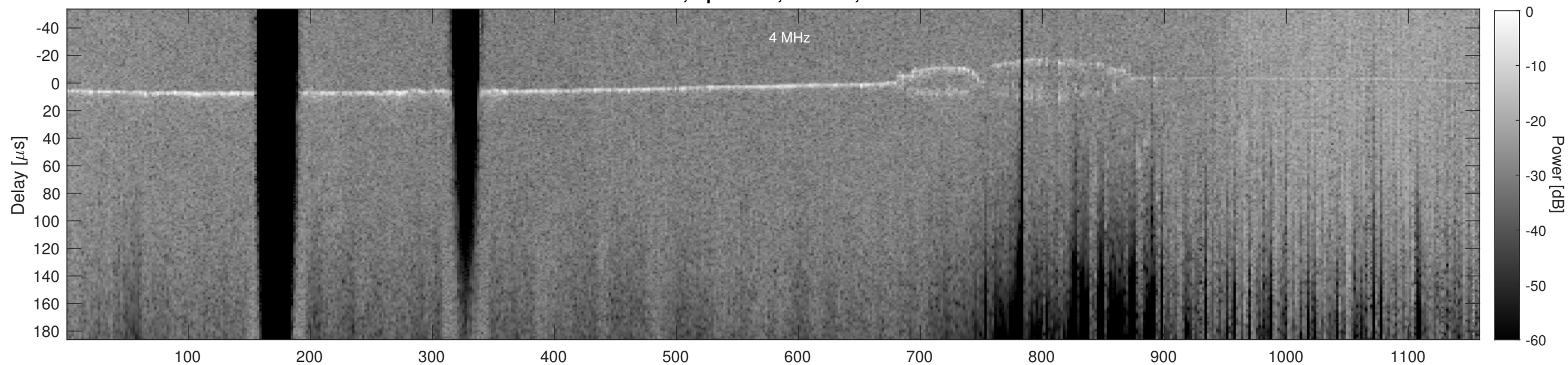
Orbit 9877, Cluttergram
