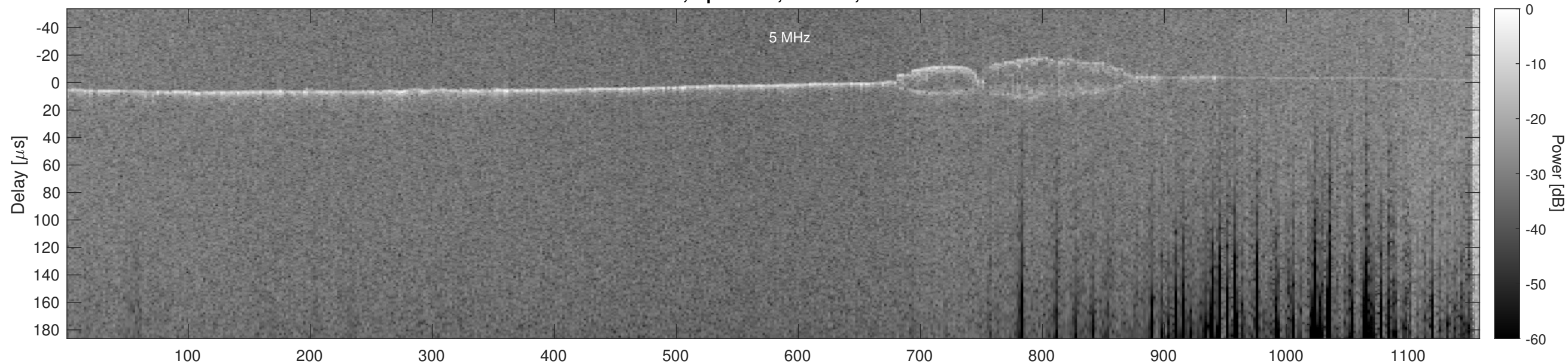
Orbit 9877, Optimized, Window, Channel 2
