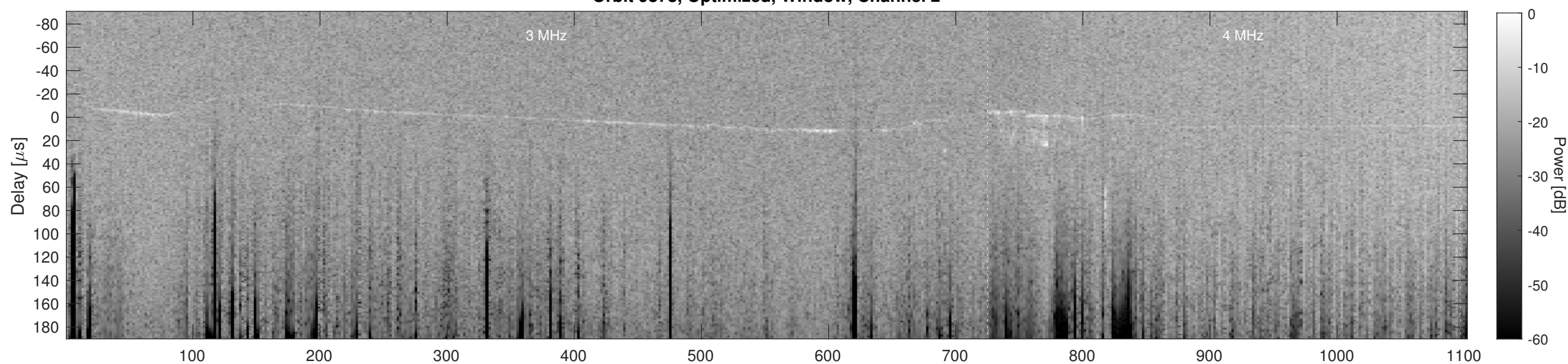
Orbit 9878, Cluttergram
