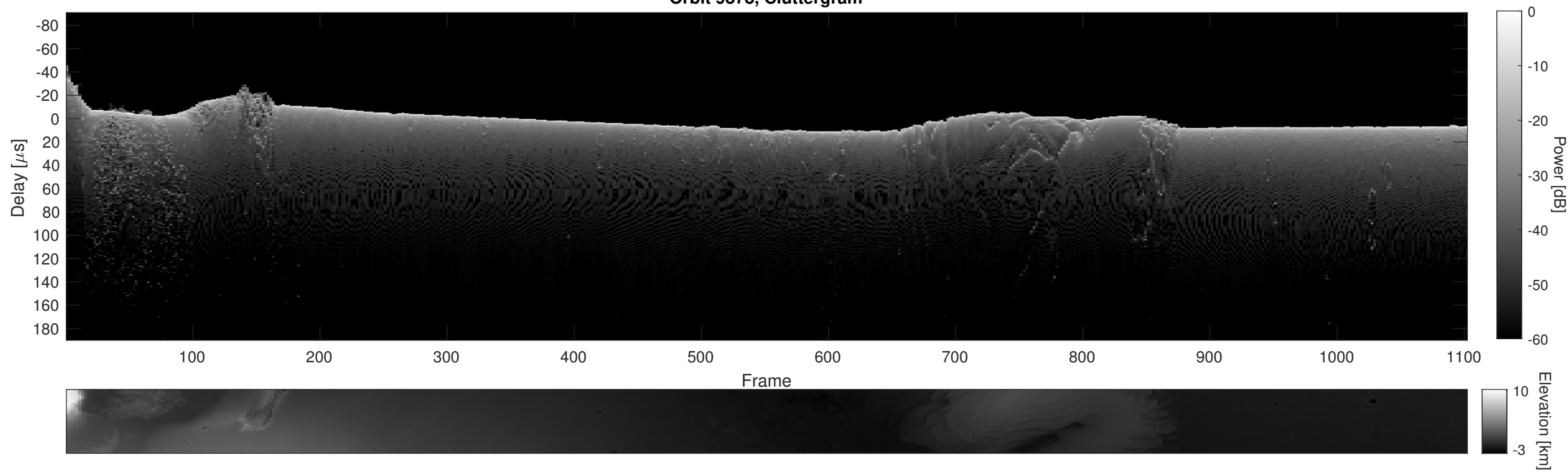
Orbit 9878, Cluttergram
