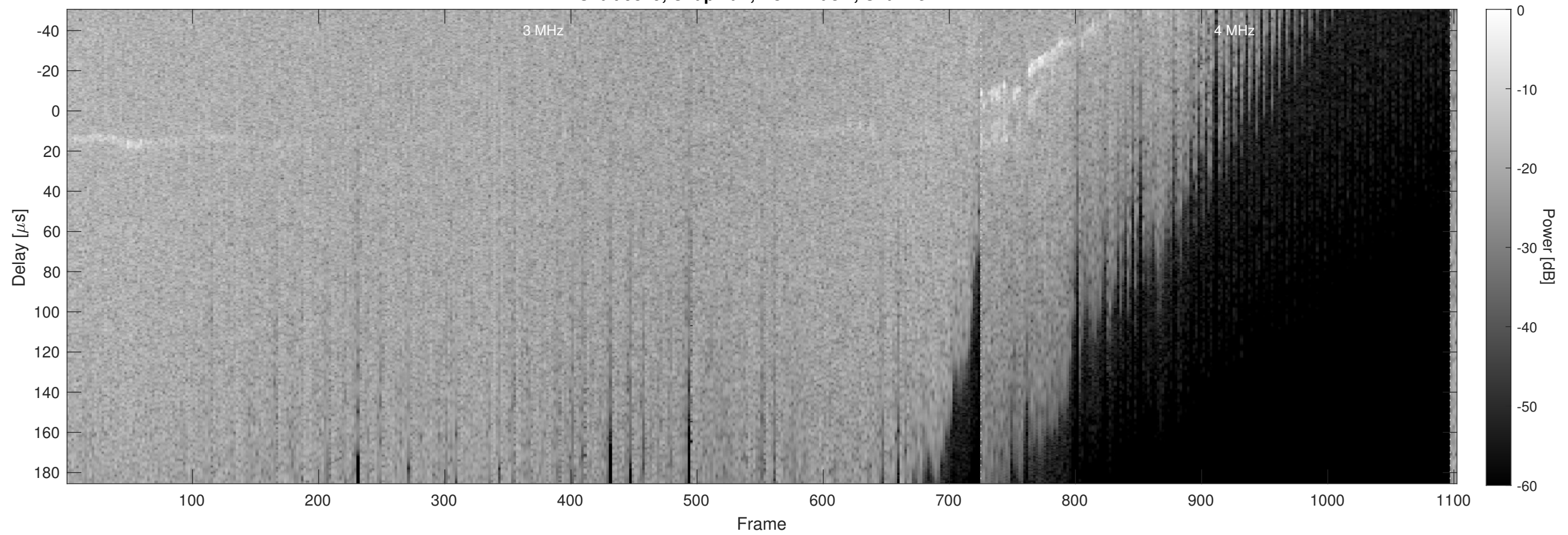
Orbit 9879, Chapman, No Window, Channel 2
