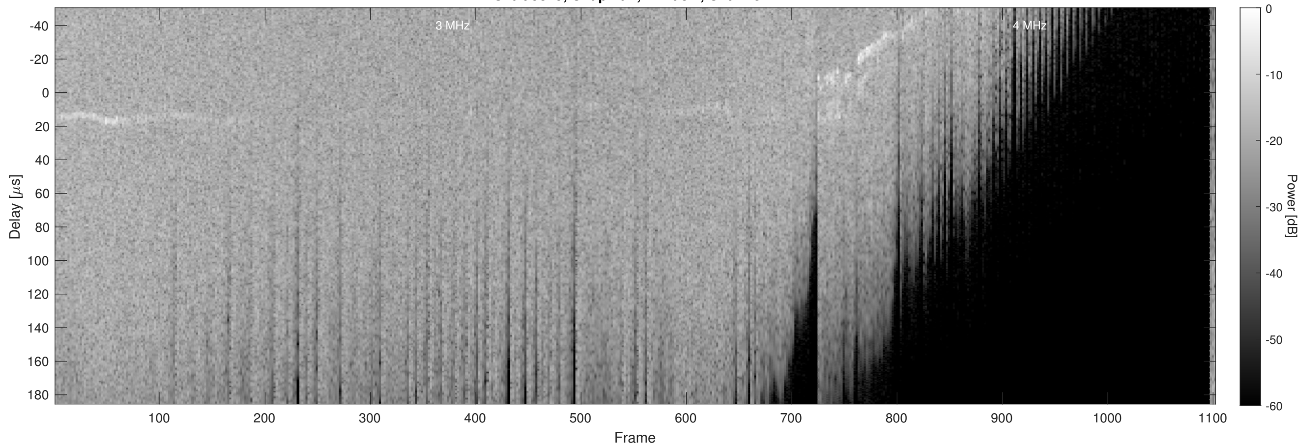
Orbit 9879, Chapman, Window, Channel 2
