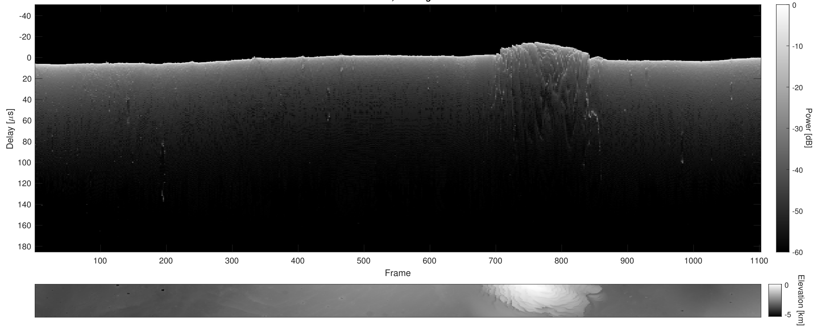
Orbit 9879, Cluttergram
