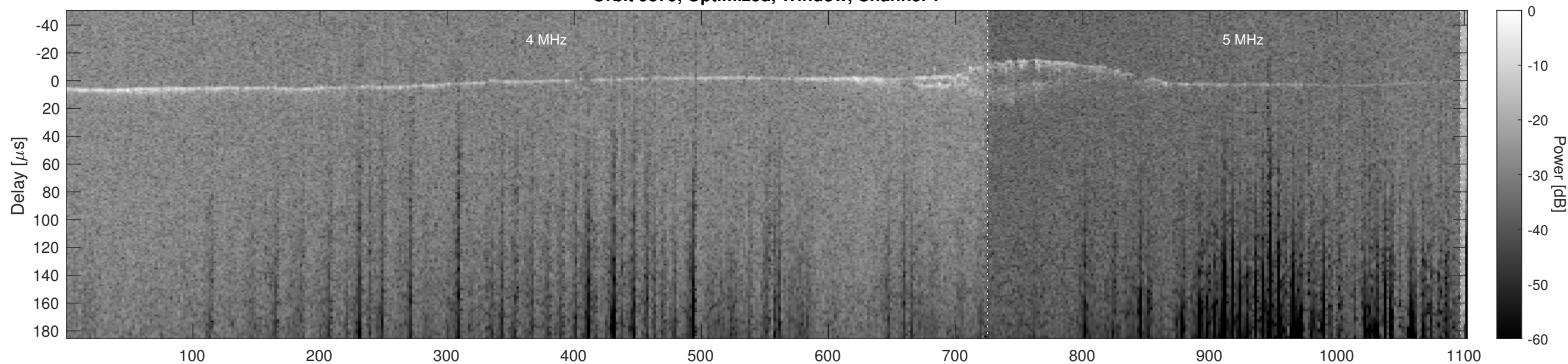
Orbit 9879, Optimized, Window, Channel 2
