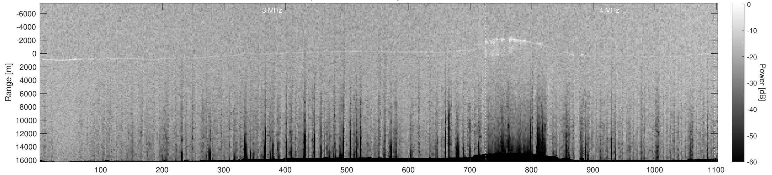
Orbit 9879, Depth-Corrected Cluttergram
