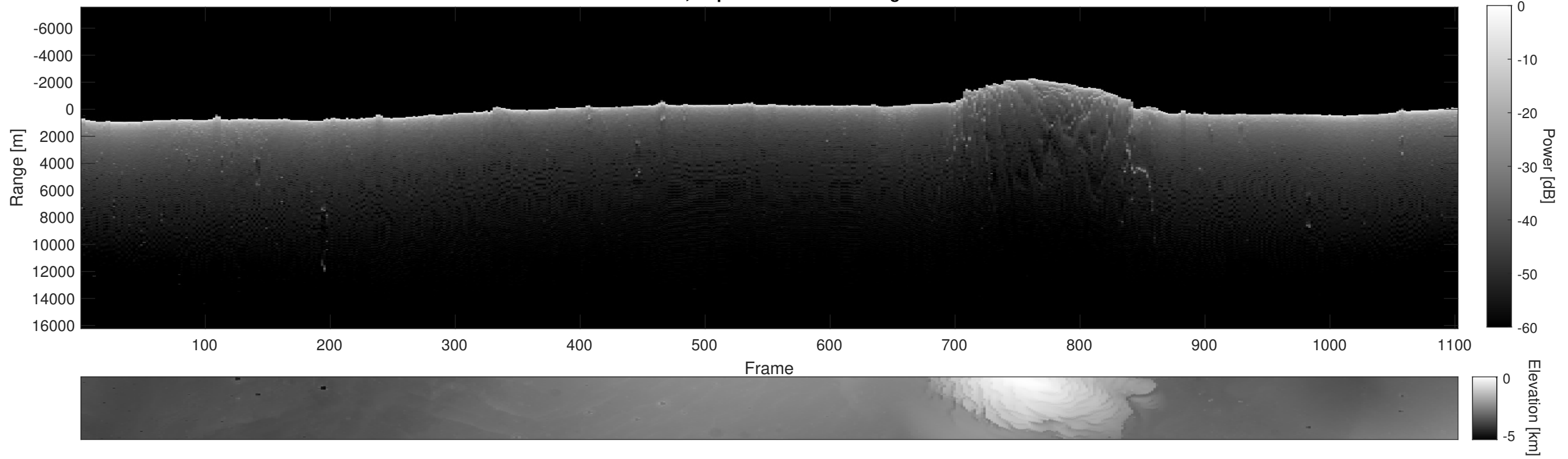
Orbit 9879, Depth-Corrected Cluttergram
